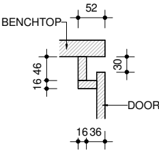
FG CUPBOARD FINGER GRIP DETAIL A105 1 : 10
