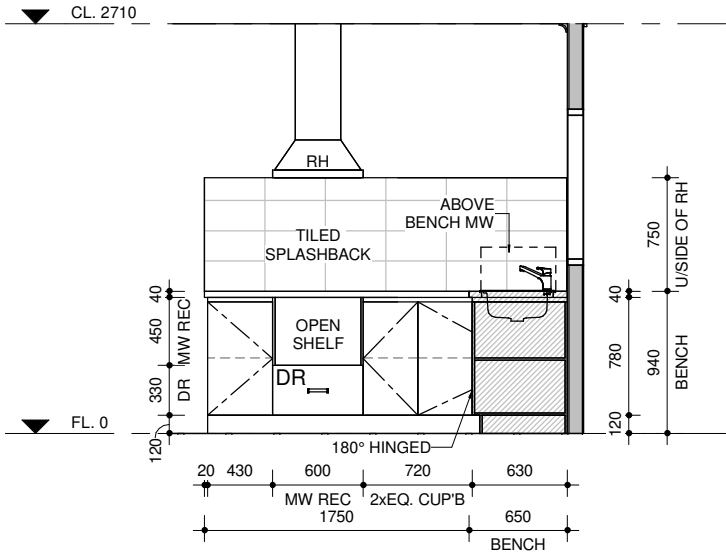
K1 K1 KITCHEN A105 1 : 50
