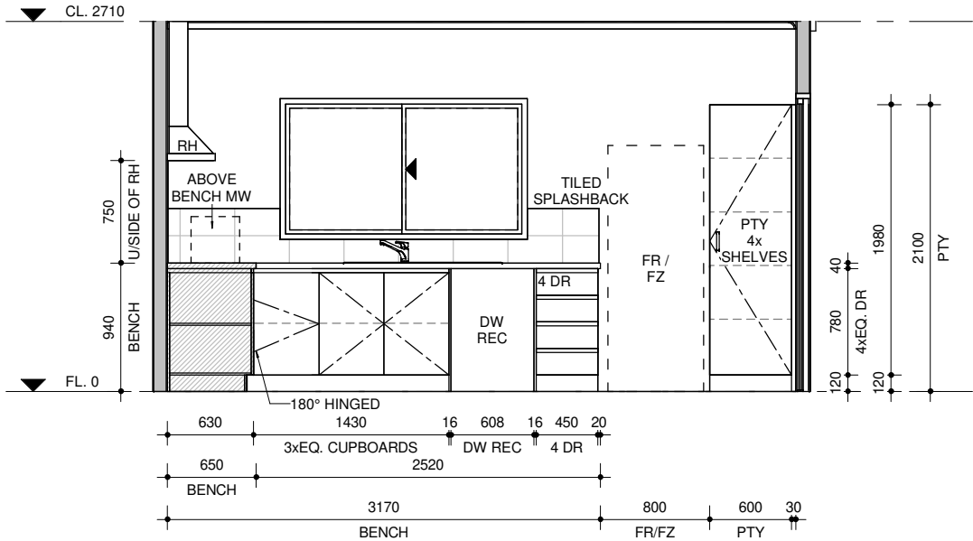
K2 K2 KITCHEN A105 1 : 50
